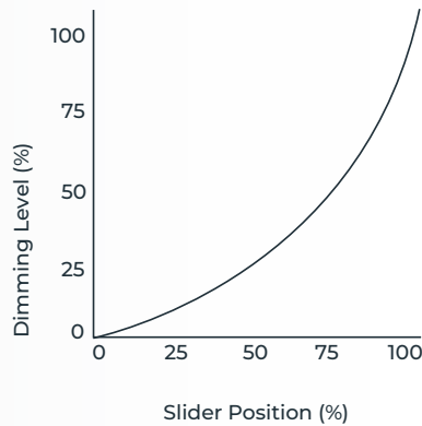
Dimming Curve
