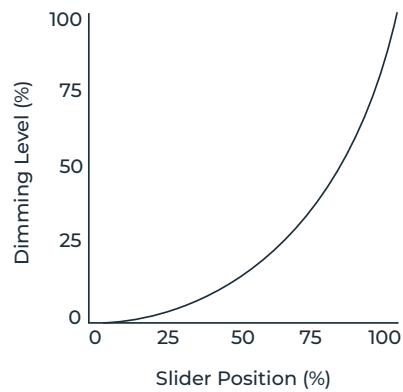
Dimming Curve
